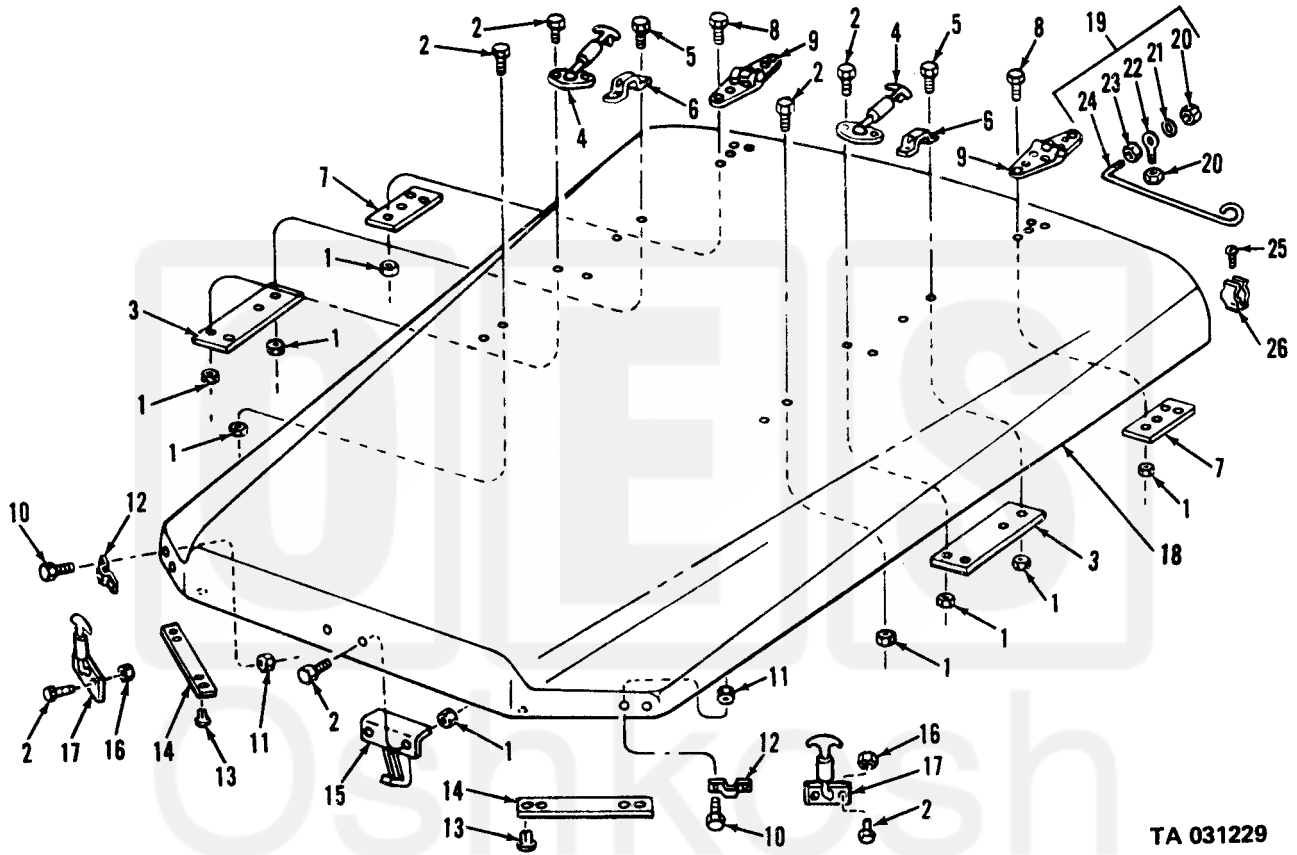
Figure 154. Hood assembly.
